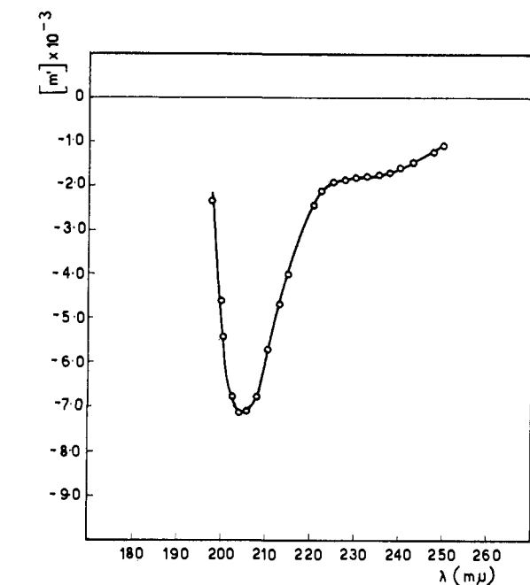
Figure 1. Far-ultraviolet ORD of [Orn 10 ,Nle 13 ]-S-peptide in water. Concentration 0.107% as determined by dry weight.
