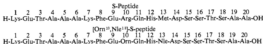
Chart I. Amino Acid Sequences of S-Peptide and [Orn 10 ,Nle 13 ]-S-peptide
